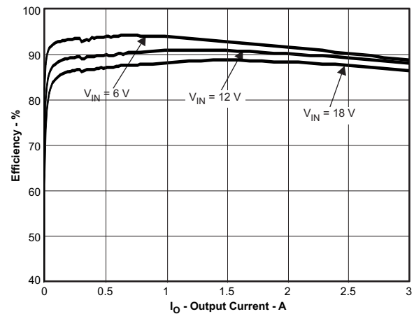
Figure 12. \text{VO1}=3.3\text{V} , Efficiency vs Output Current
