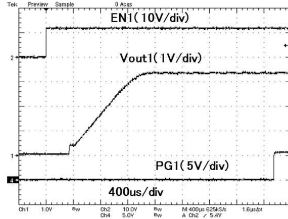
Figure 10. \text{VO1}=3.3\text{V} , PG
