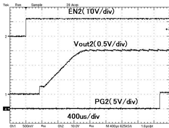
Figure 11. \text{VO2}=1.5\text{V} , PG
